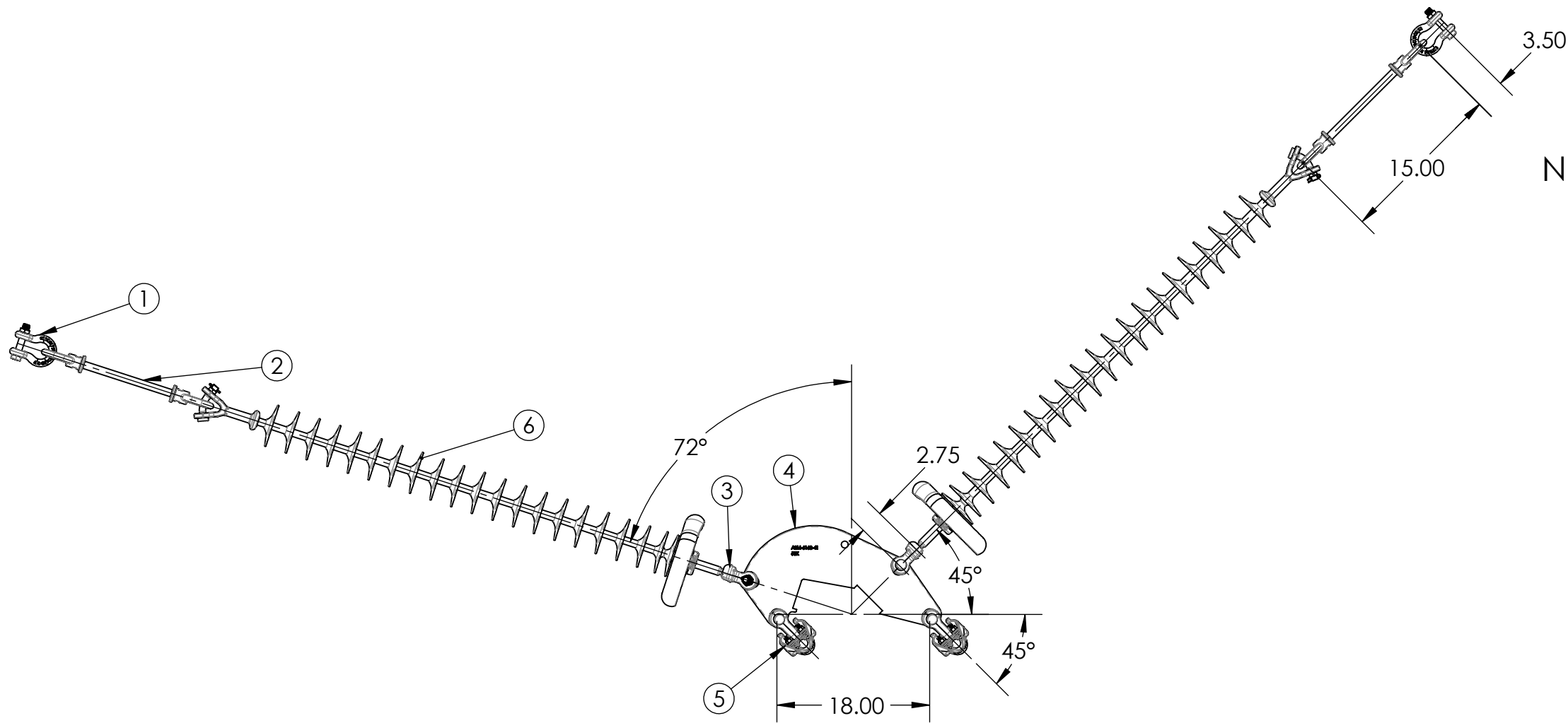
ASSEMBLY CAT. NO. X3RV2YB30B2
